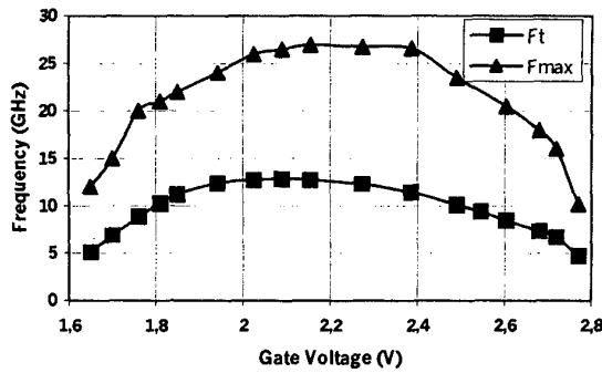
Fig. 5. Current gain and maximum available gain cutoff frequencies versus gate voltage at 12 V DC supply voltage. Highest value of f_{MAX} coincide with the bias for highest gm, while maximum f_T is achieved for somewhat lower bias.
