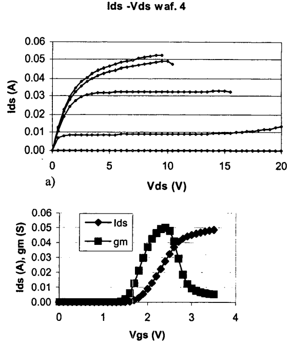
Fig. 3. I - V characteristics of LDMOS transistor with a total gate width of 0.4 mm, and extended drain region of 1 \mu\text{m} a) I_{ds} vs. V_{ds} for V_{gs} = 1 - 3.5 V in 0.5 V steps, b) I_{ds} & g_m vs. V_{gs} at V_{ds} = 6 V, V_{th} = 1.8 V
